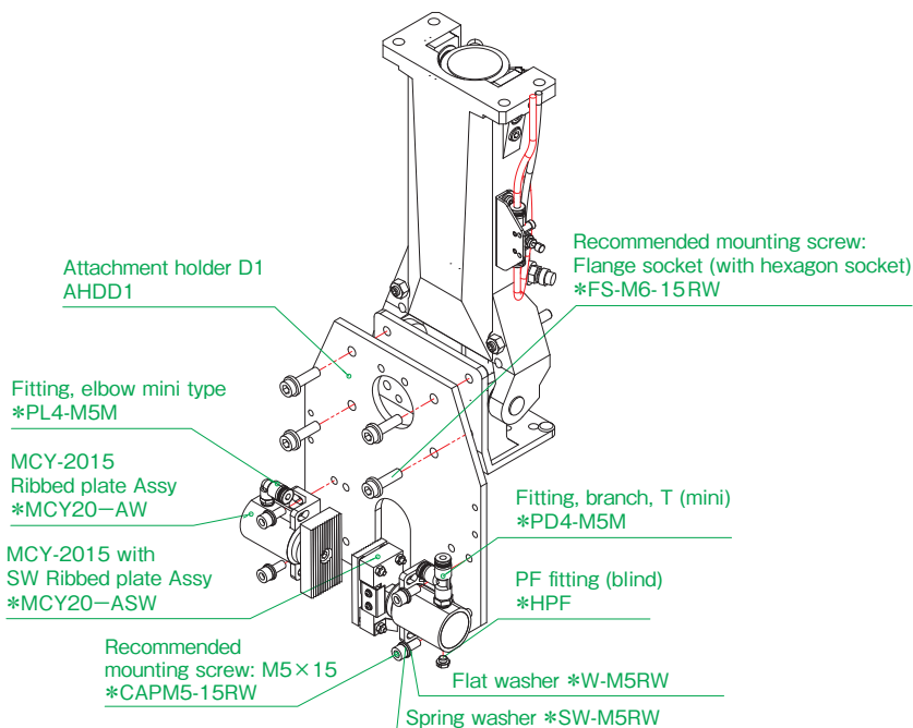
Usage example of AHDD1: Gripper type, for traverse-type robot
