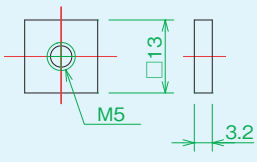
Rail mounting bracket (13×13)
