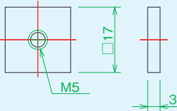
Rail mounting bracket (17×17)
