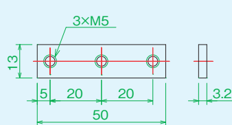
Rail mounting bracketNo.6
