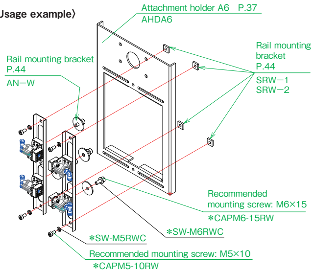
Washer for rail
